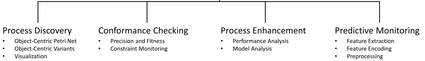
Figure 1: Overview for the functionalities contained in OCPA.
